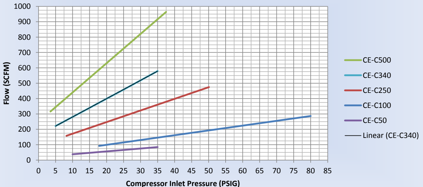
Suction pressure vs. flow for various Cobey Energy models
